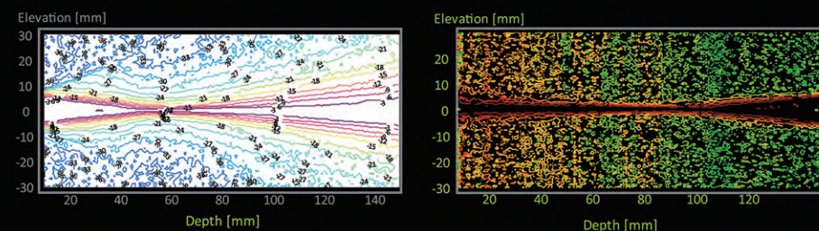
Traditional Probe
